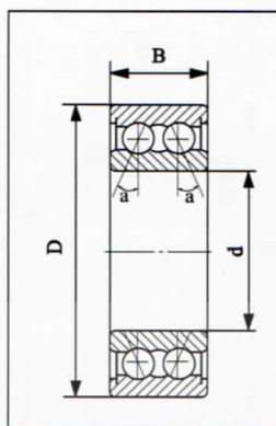
5000 ZZ (3000 ZZ) 5000-2RS (3000-2RS)
