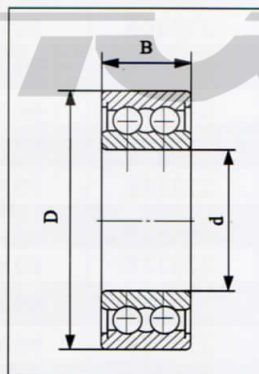
4000 ZZ 4000 2RS
